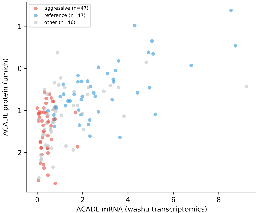
ACADL RNA-protein concordance — umich Spearman rho=0.627, p=1.19e-16
