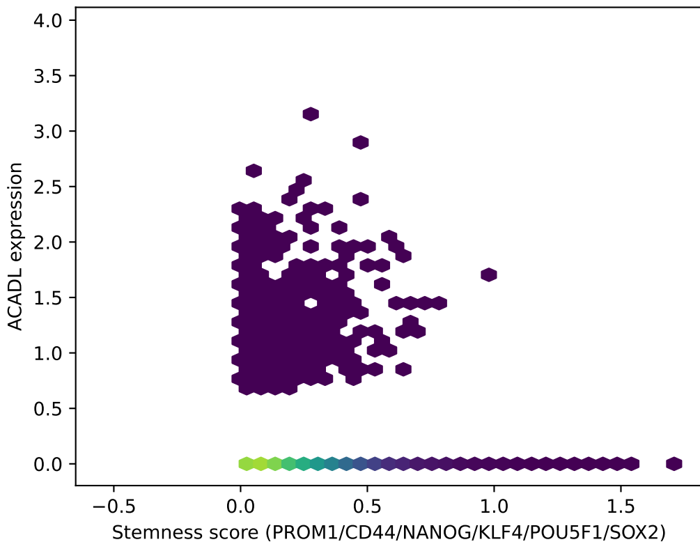
GSE202051: ACADL vs stemness (malignant cells)
