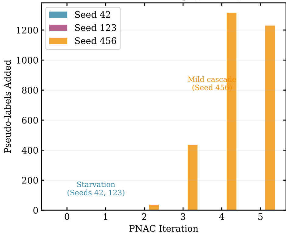
(B) Pseudo-label Throughput at \rho = 0.55
