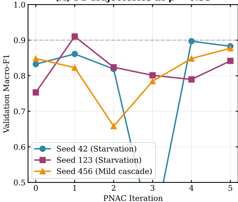
(A) F1 Trajectories at \rho = 0.55
