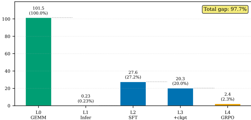
Achieved TFLOPS
