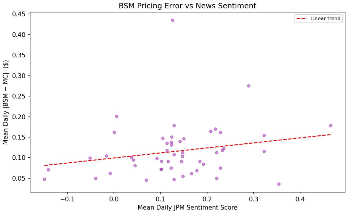
Sentiment Scatter
