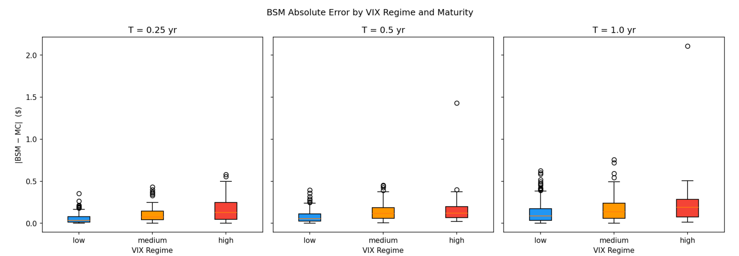
Regime Boxplot
