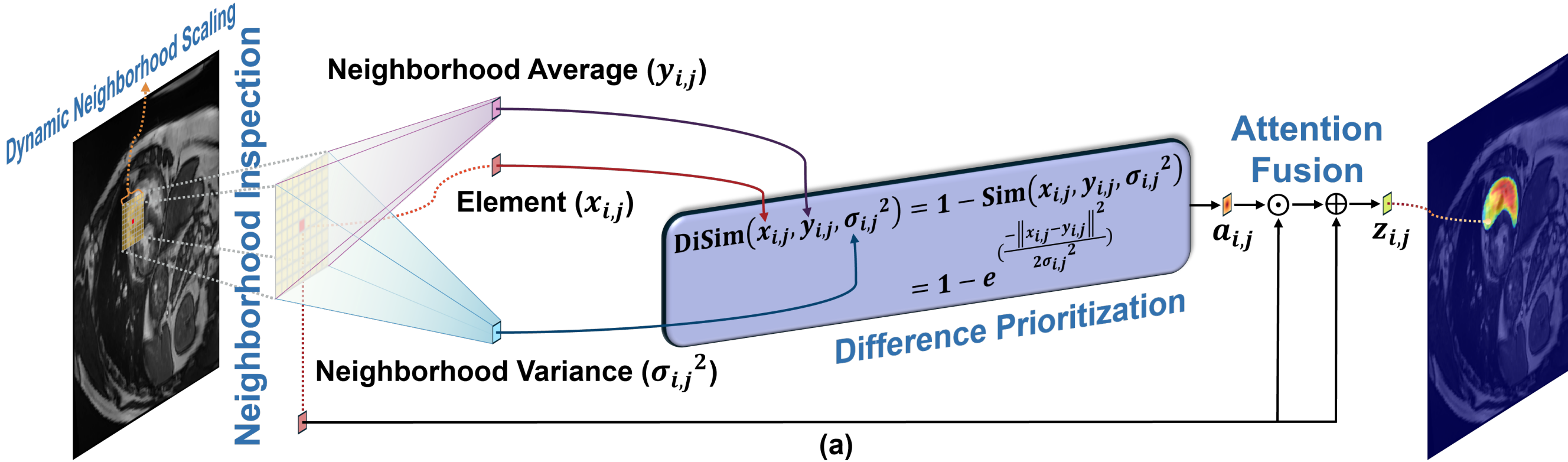
Gaussian-Kernel-Based Dissimilarity
