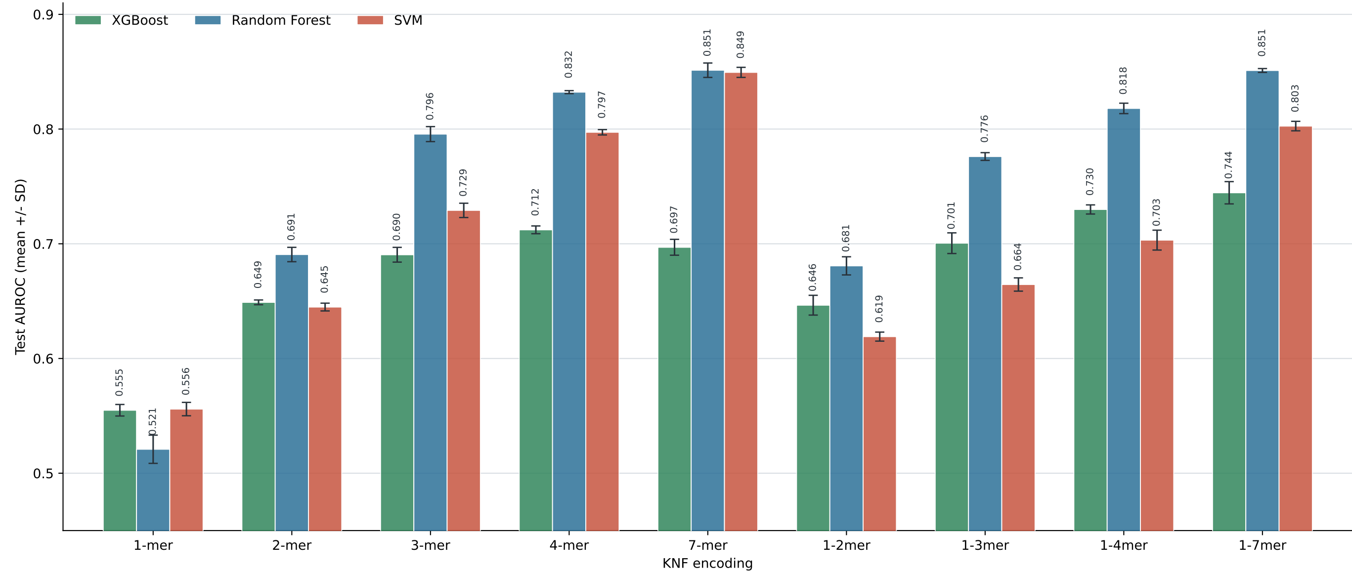
Classical classifiers across three stratified random 80/20 splits
