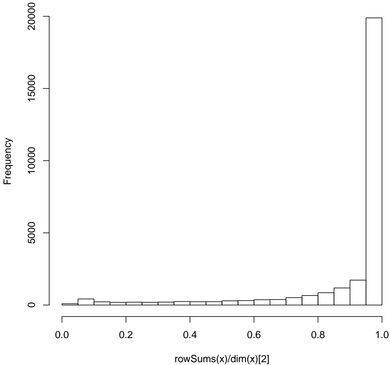
Histogram of rowSums(x)/dim(x)[2]
