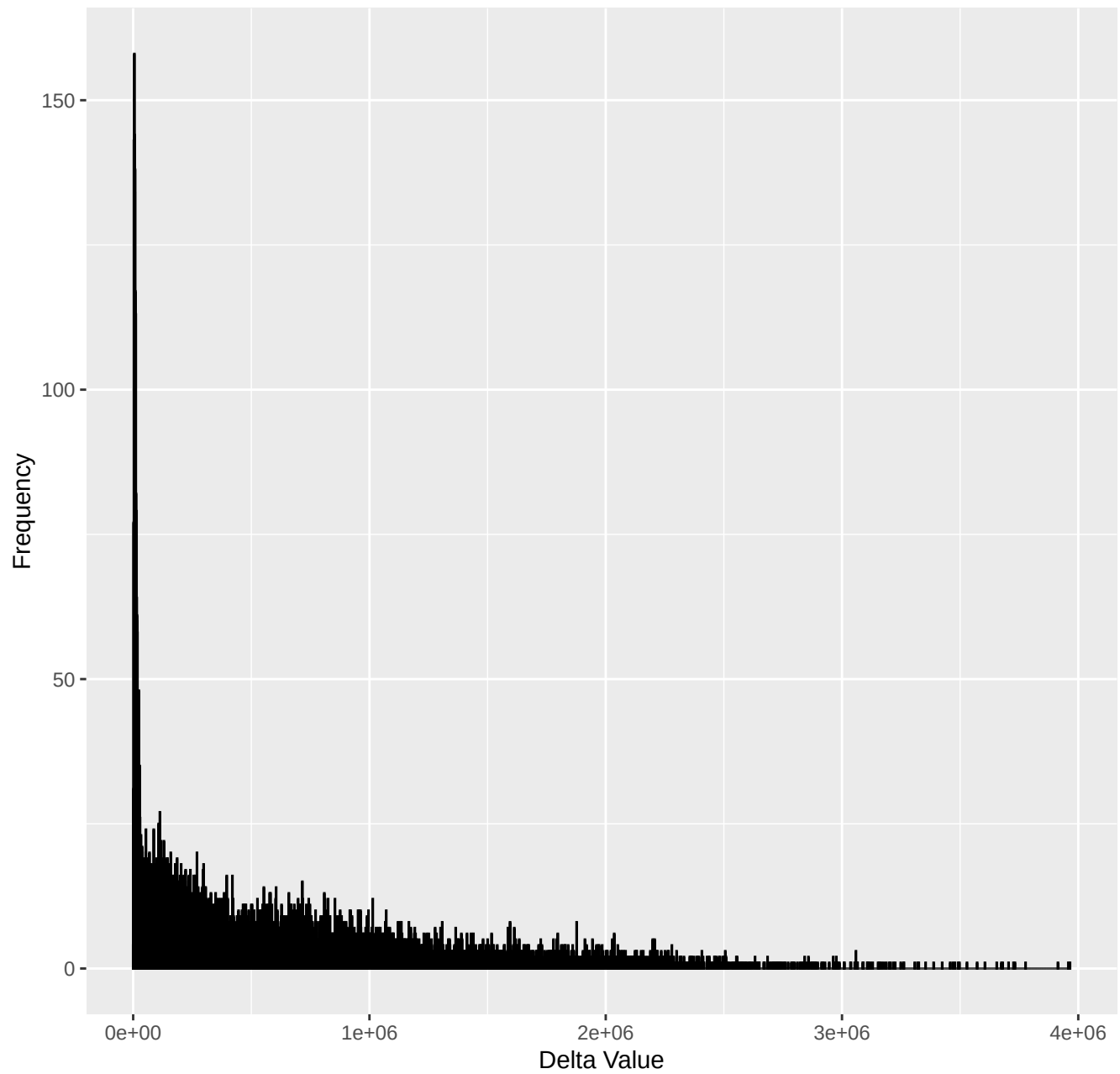
Distribution of Delta Band
