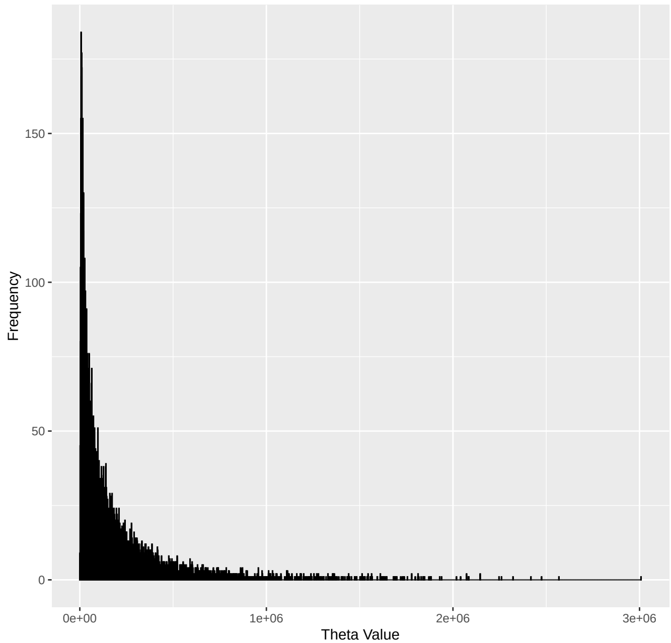
Distribution of Theta Band
