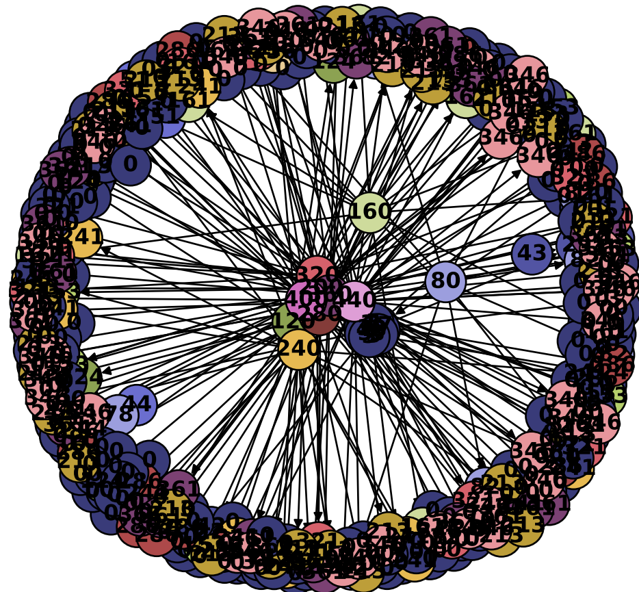
Graph Colored by Orbit Labels
