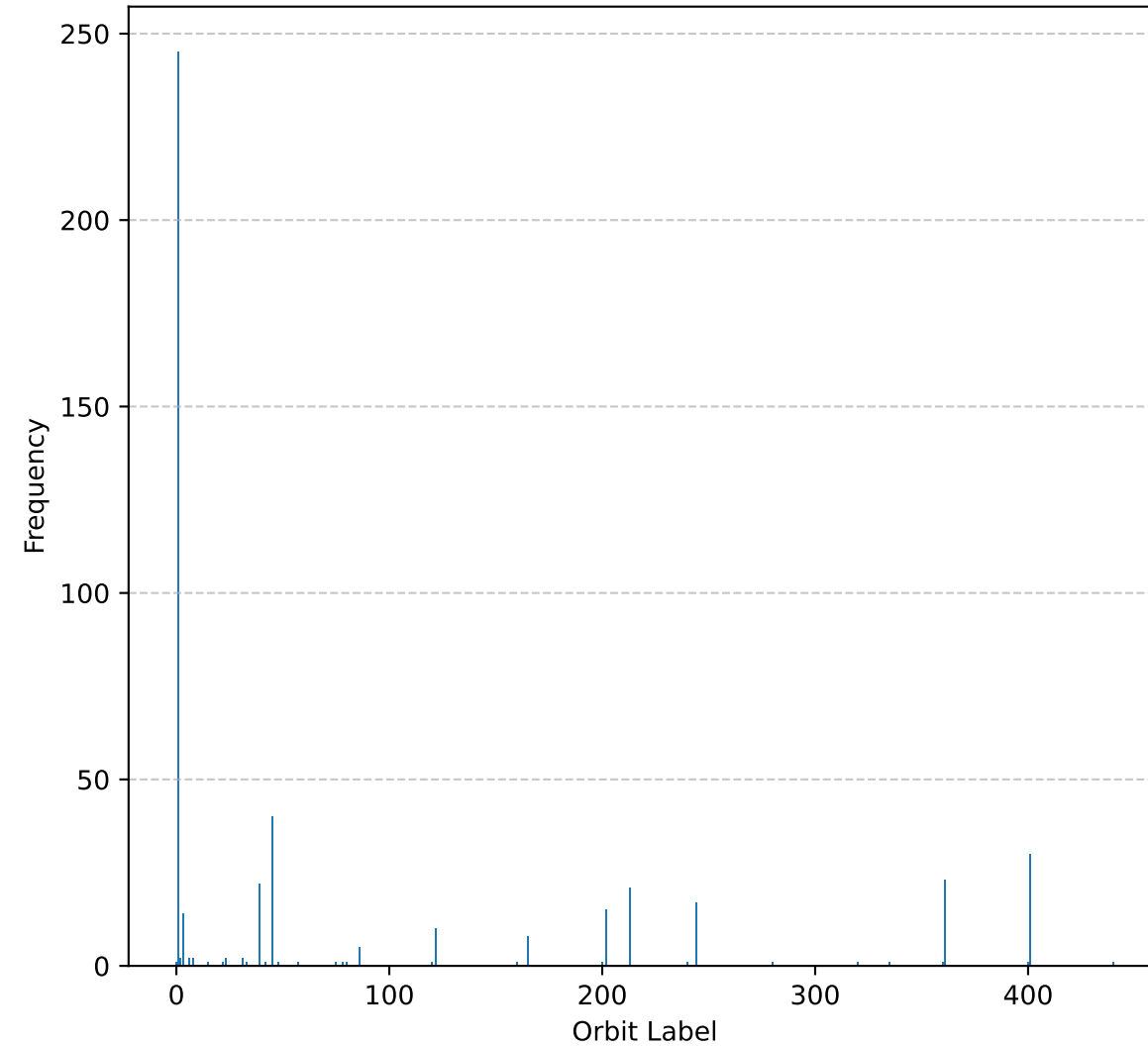
Orbit Distribution
