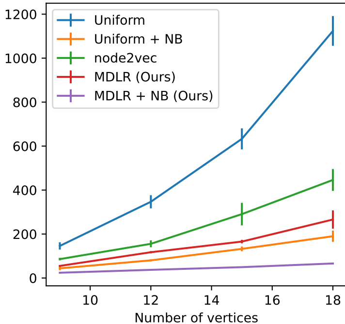
Vertex cover time C_V(G)
