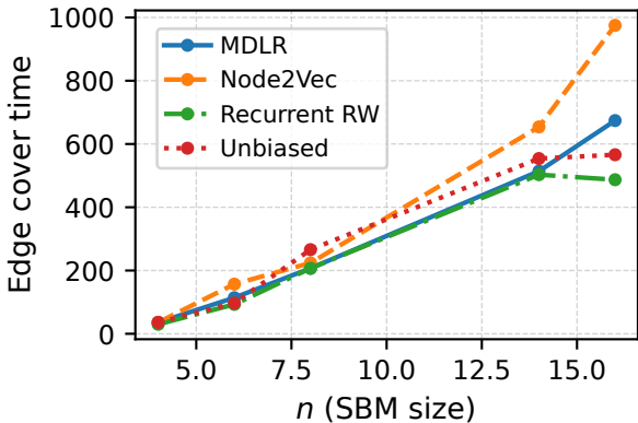
Edge Cover Time vs n on SBM graphs
