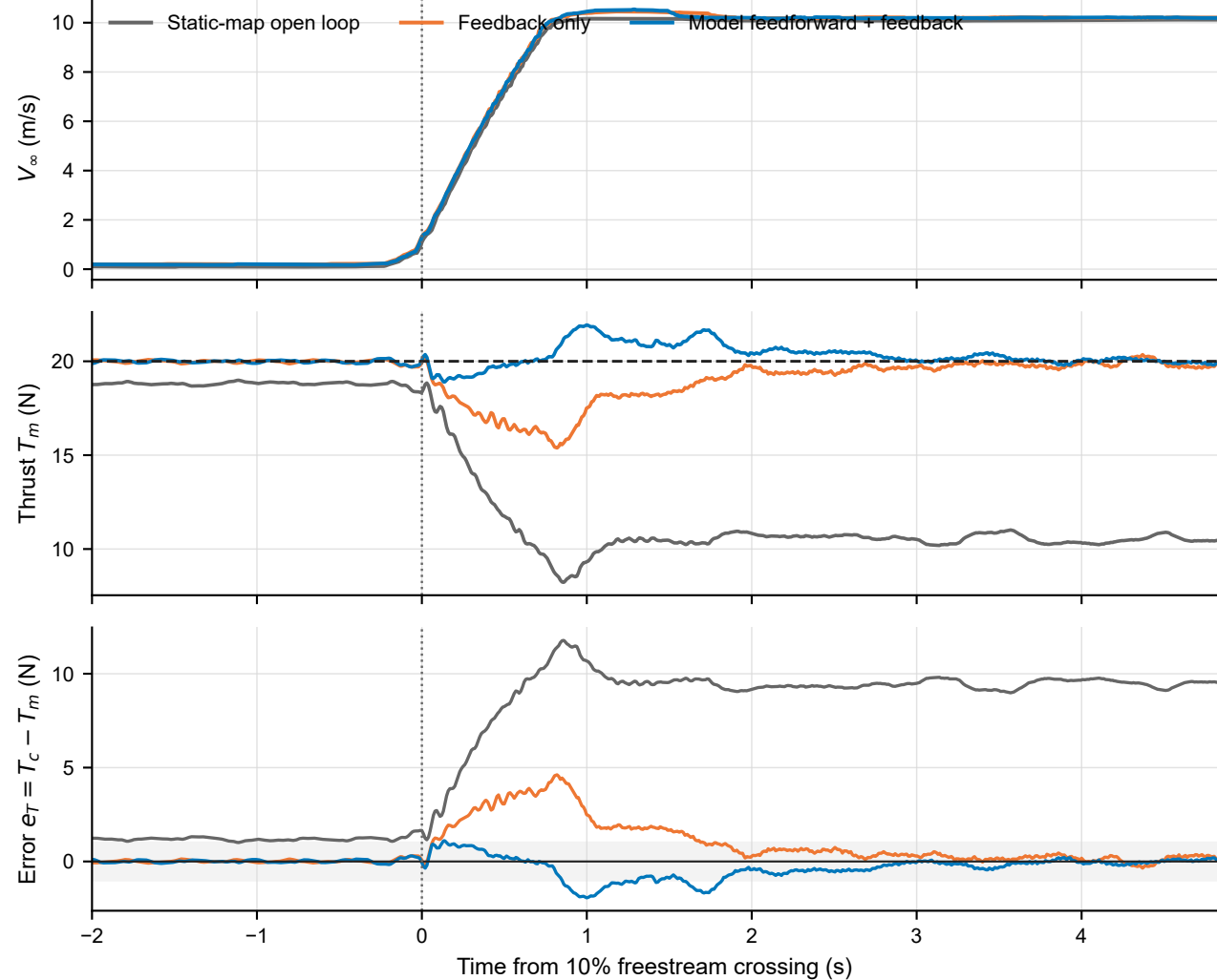
20 N target, nominal 1 s acceleration: aligned dynamic response
