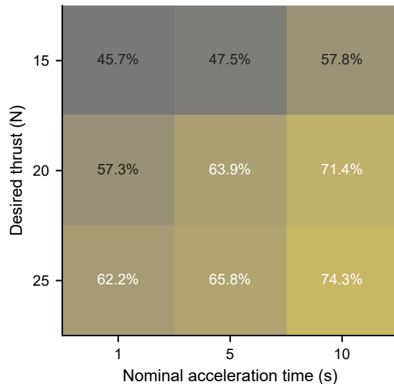
(b) Model FF + feedback vs feedback: RMSE reduction
