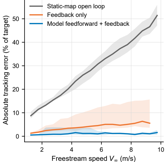
(c) Error over the freestream-speed sweep
