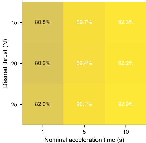
(a) Feedback vs static: RMSE reduction
