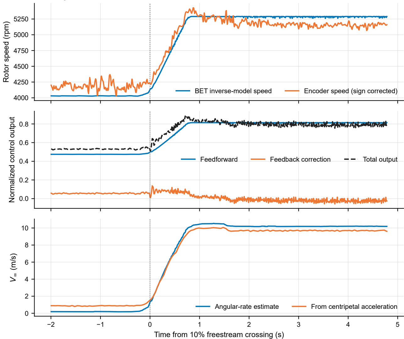
20 N target, nominal 1 s acceleration: feedforward mechanism checks
