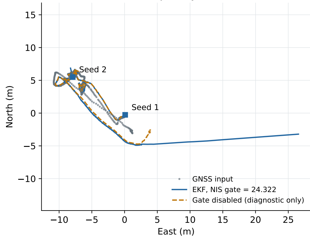
Horizontal trajectory in local ENU
