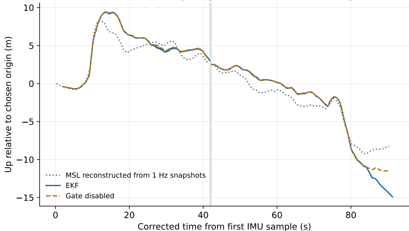
Vertical trajectory; original GPS altitude is missing
