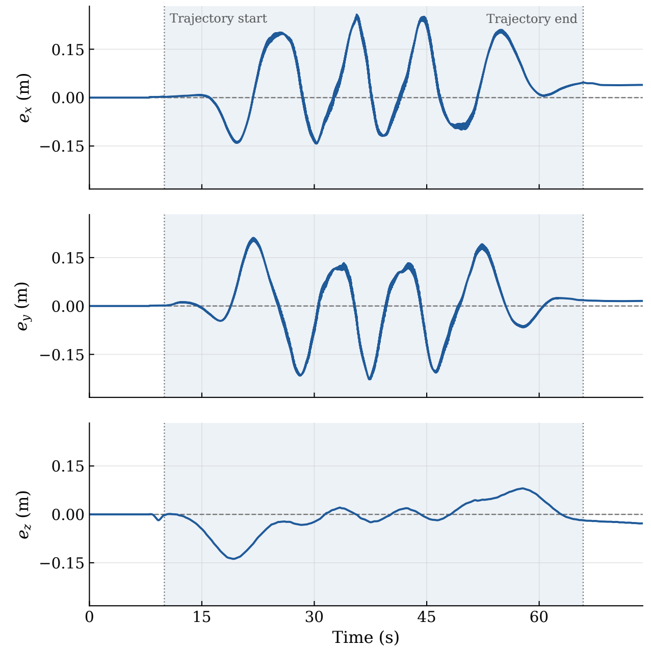
(b) Position error (actual – reference)
