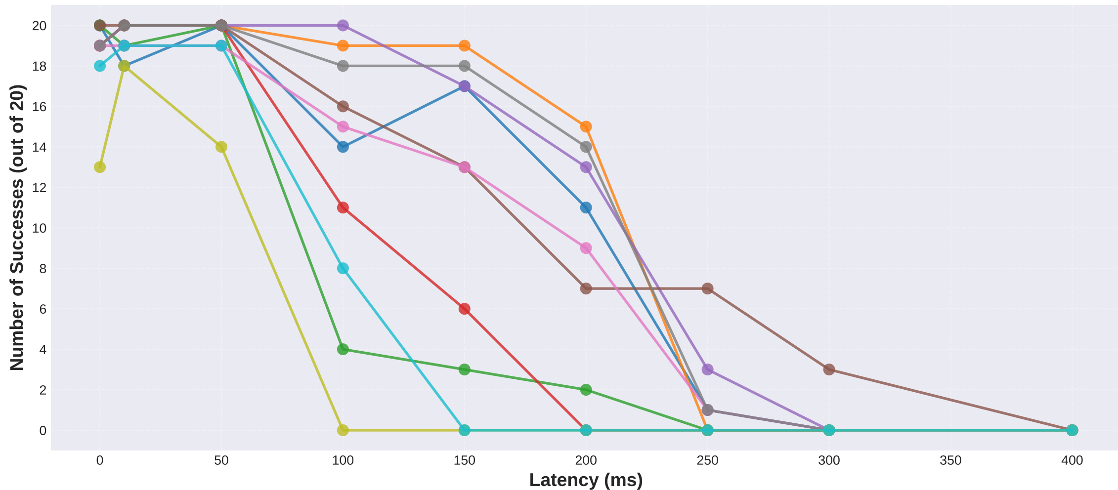
Task Success vs Latency
