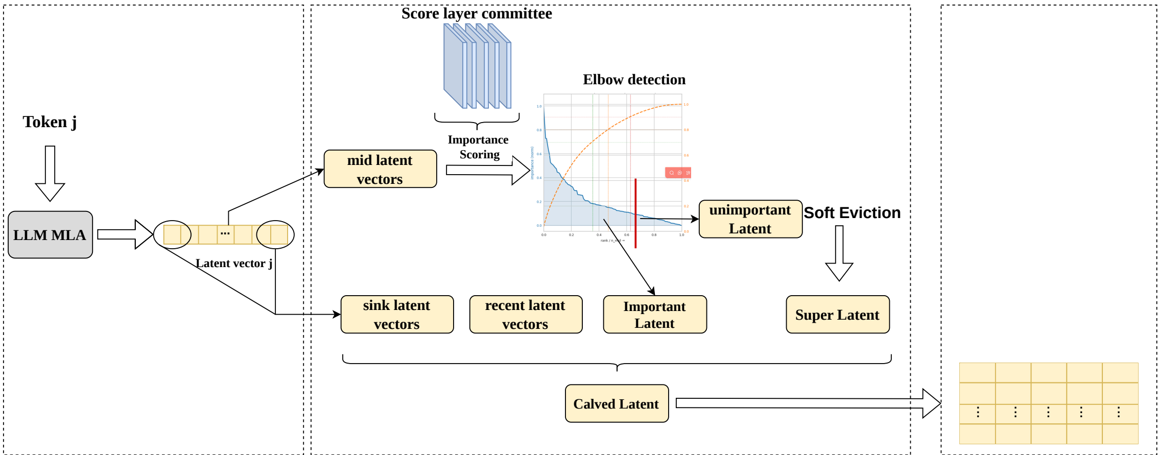
MLA algorithm
