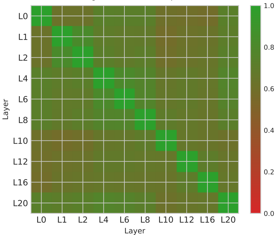
Cross-Layer Jaccard Keep-Set Overlap (top-30%) (averaged over 10 code sequences)
