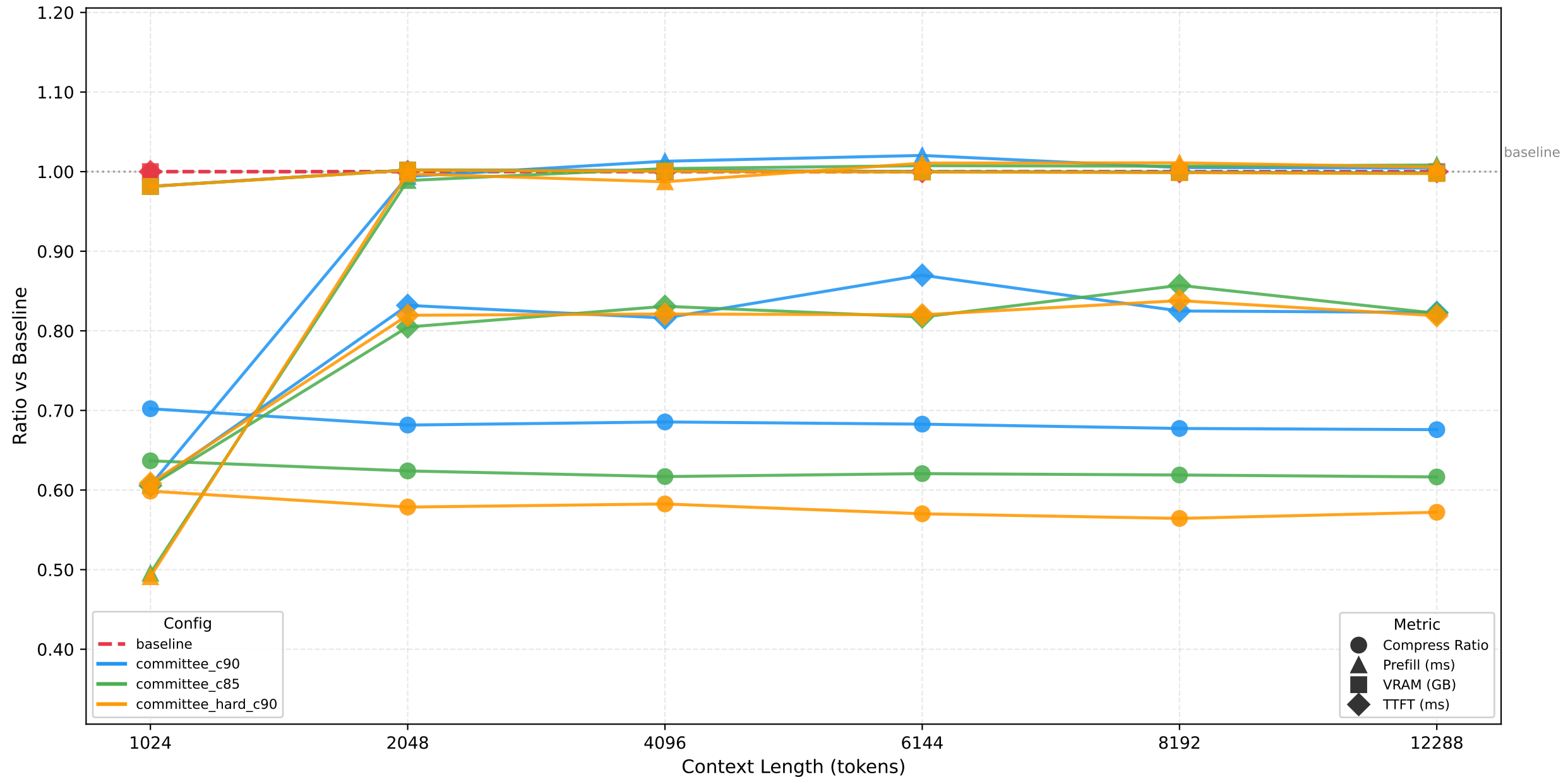
System Metrics — DeepSeek Latent Eviction (normalized to baseline)
