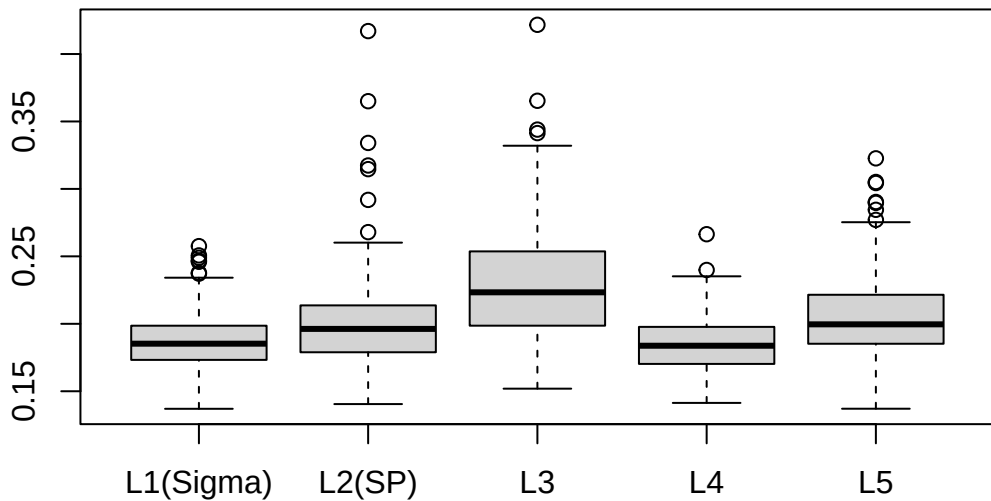
Figure 3(d): Wing Weight
