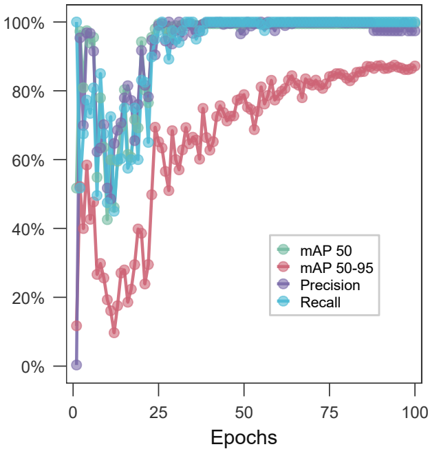
Training metrics in SVDs
