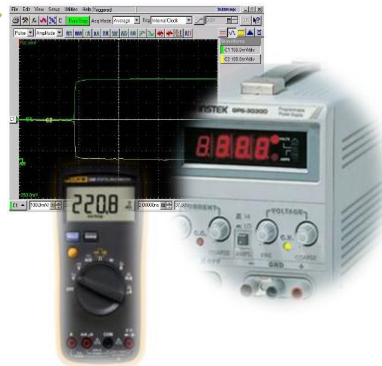
Electrical test-電性測試
