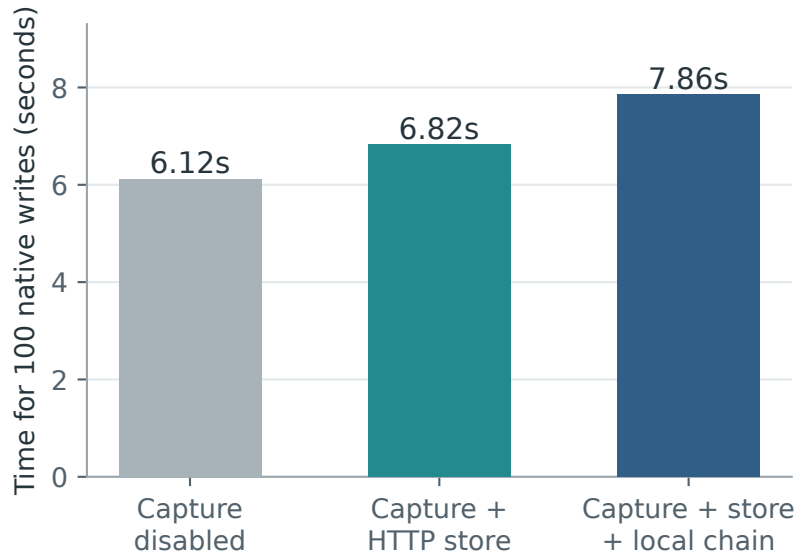
(a) Runtime overhead
