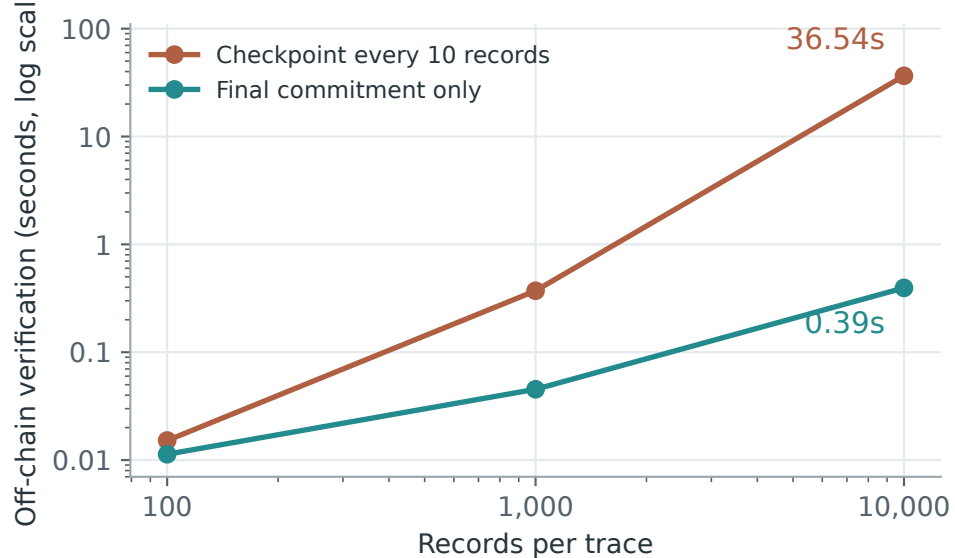
(b) Cost of cumulative prefix checks
