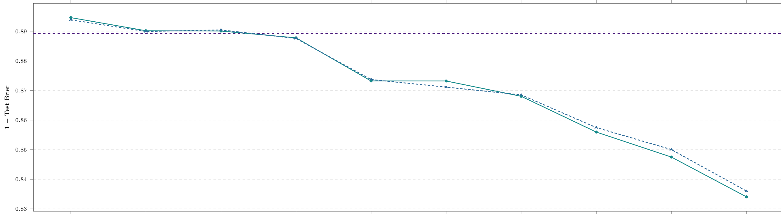
Politics - threshold 1,000 - group 37 - d375bcca520b... 6 models, 1,129 common events, 1,994 test instances, 10 Brier-weak pairs - - Best individual (Claude-3-5-Sonnet) — Our log-odds - - Learned probability pool
