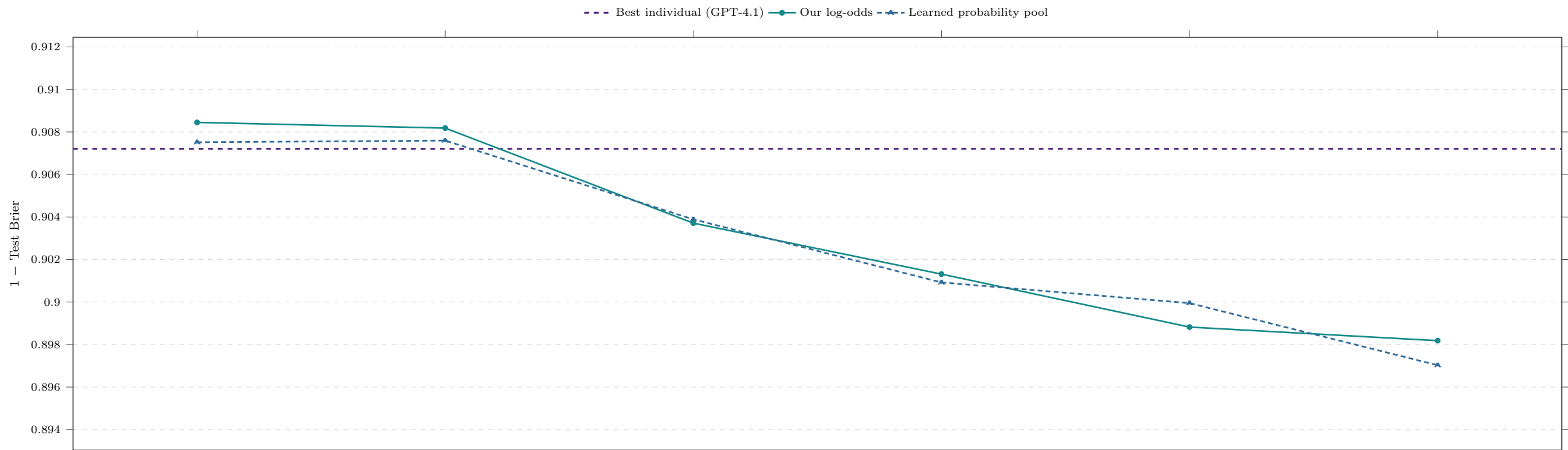
Politics - threshold 1,000 - group 40 - dfd9d5403b04... 5 models, 1,003 common events, 1,898 test instances, 6 Brier-weak pairs
