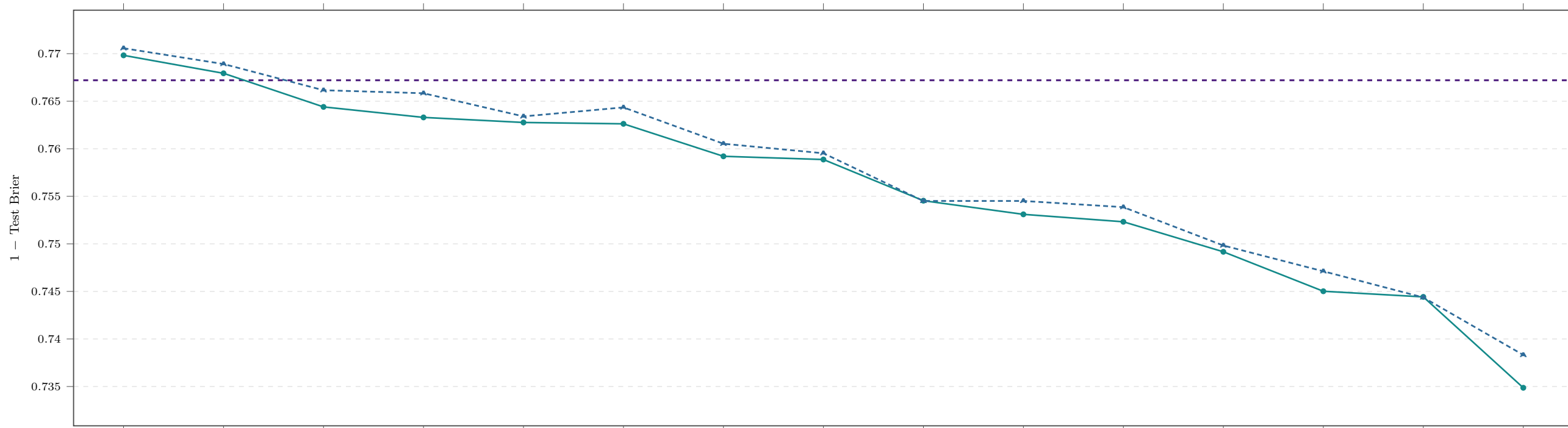
Finance - threshold 1,000 - group 07 - 5e945acef2e2... 7 models, 1,157 common events, 2,105 test instances, 15 Brier-weak pairs Best individual (Magistral-Medium) Our log-odds Learned probability pool
