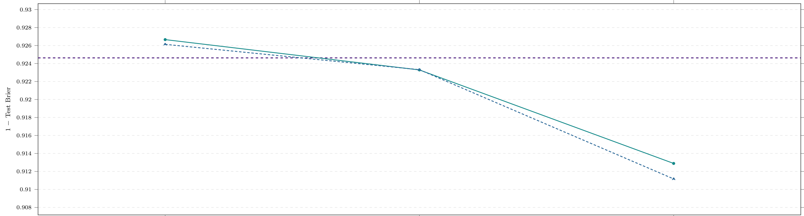
Politics - threshold 1,000 - group 43 - b20f0bd9508a... 4 models, 1,071 common events, 1,464 test instances, 3 Brier-weak pairs - - - Best individual (GPT-5-Mini) —●— Our log-odds - -▲- Learned probability pool
