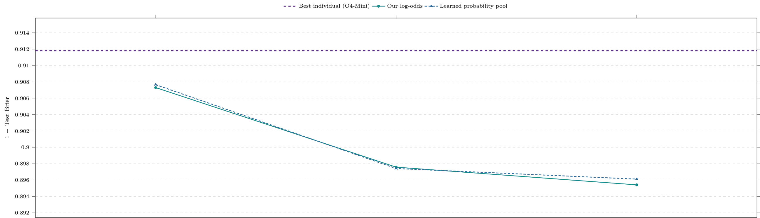
Politics - threshold 1,000 - group 41 - f18f46c4388c... 4 models, 1,313 common events, 2,398 test instances, 3 Brier-weak pairs
