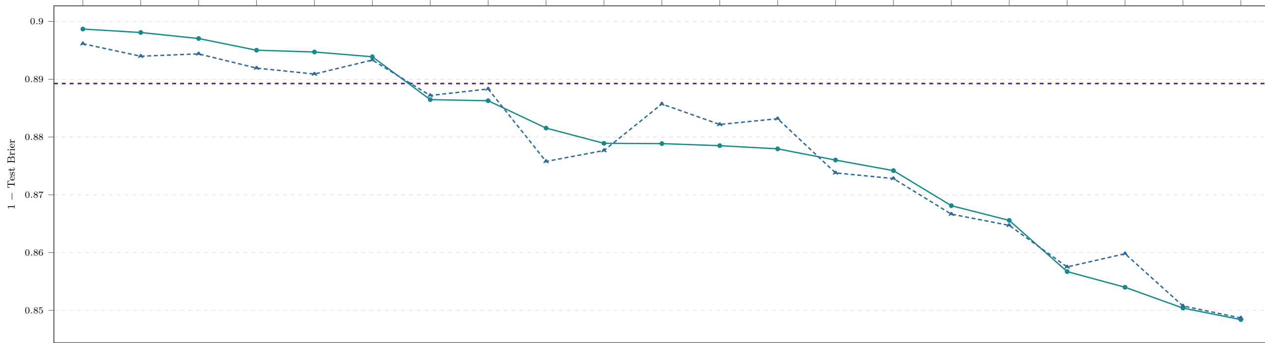
Politics - threshold 1,000 - group 35 - 0ff3b243f647... 8 models, 1,035 common events, 1,606 test instances, 21 Brier-weak pairs Best individual (Claude-3-5-Sonnet) Our log-odds Learned probability pool
