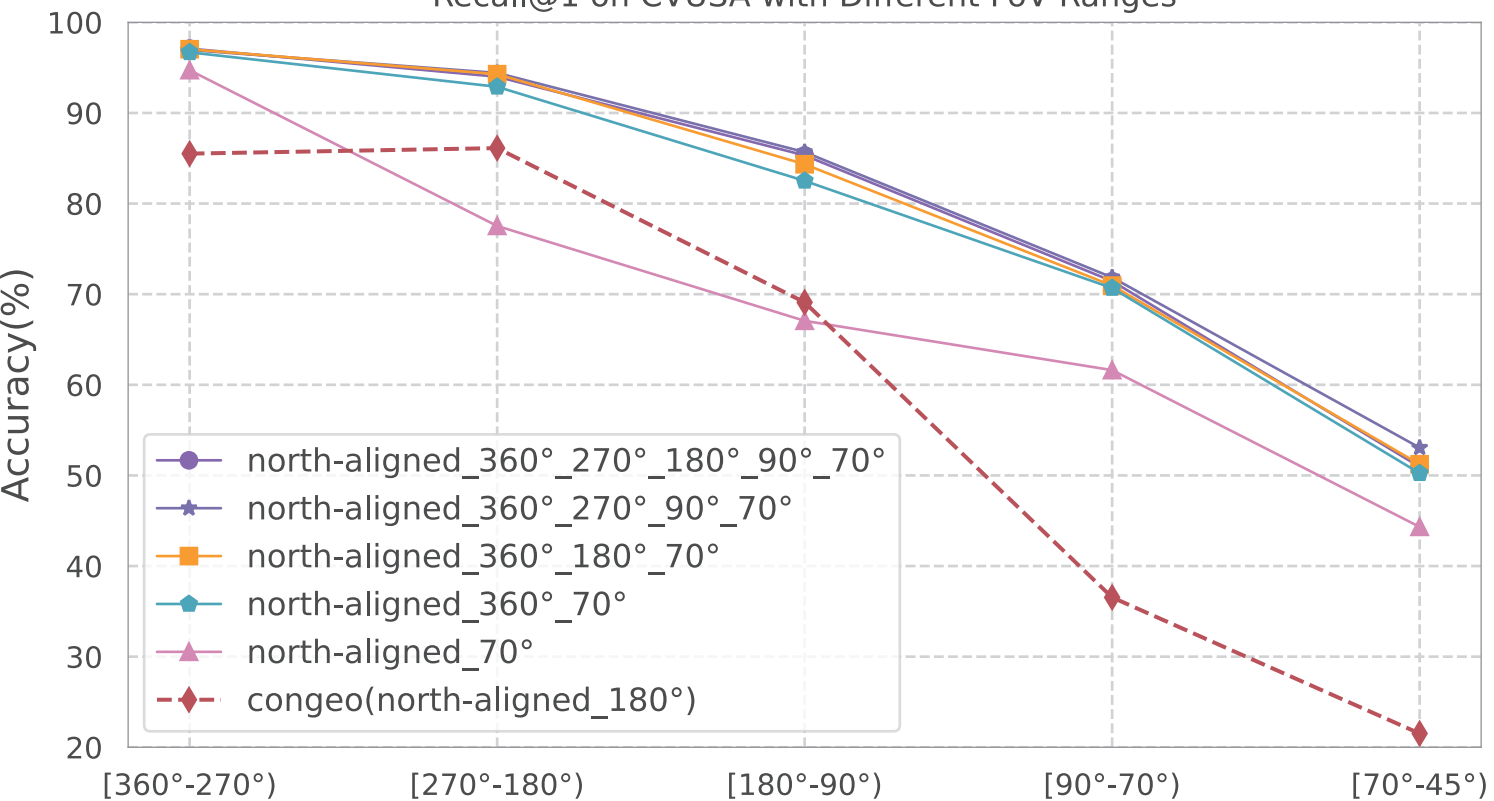
Recall@1 on CVUSA with Different FoV Ranges
