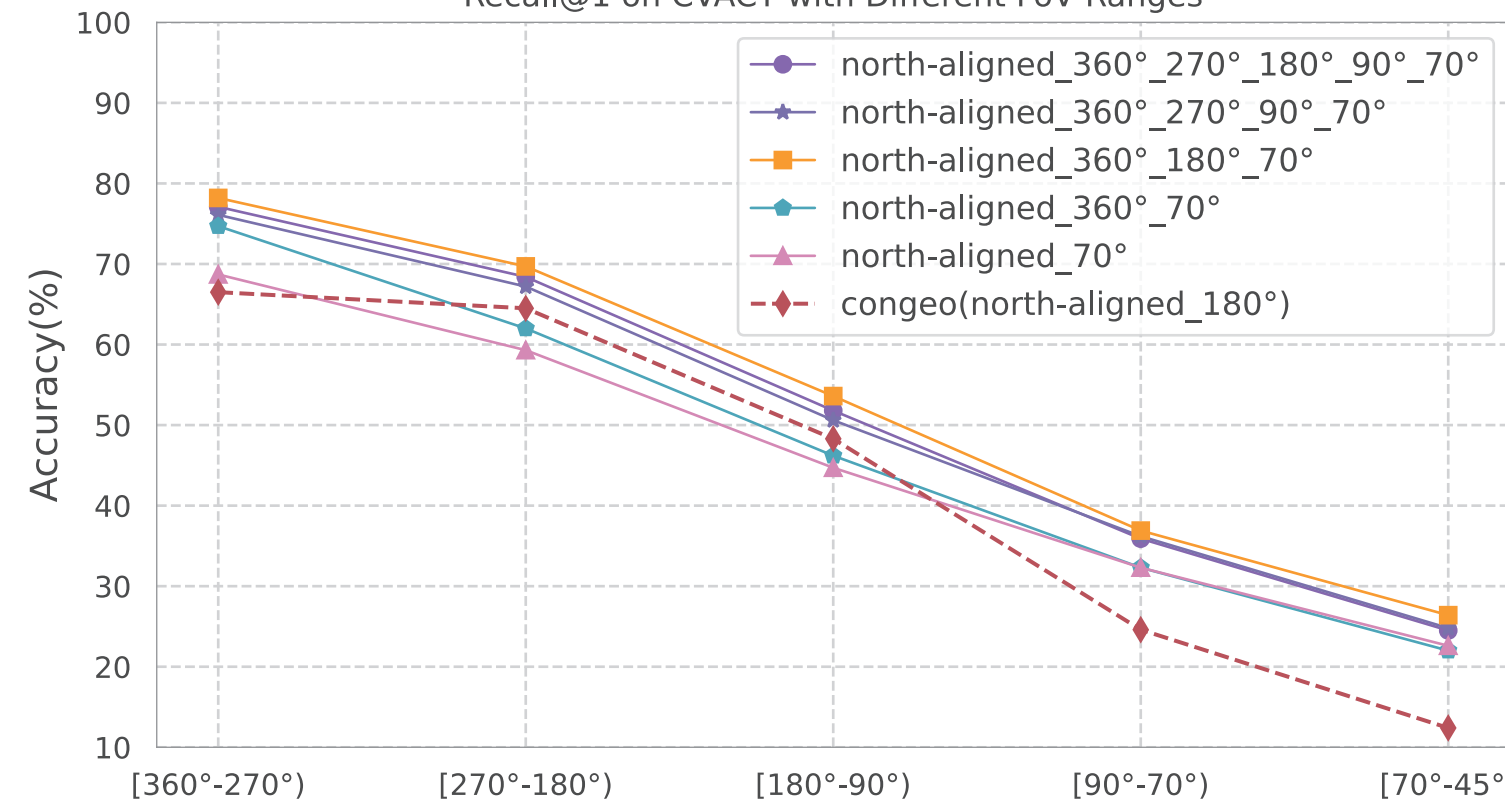
Recall@1 on CVACT with Different FoV Ranges
