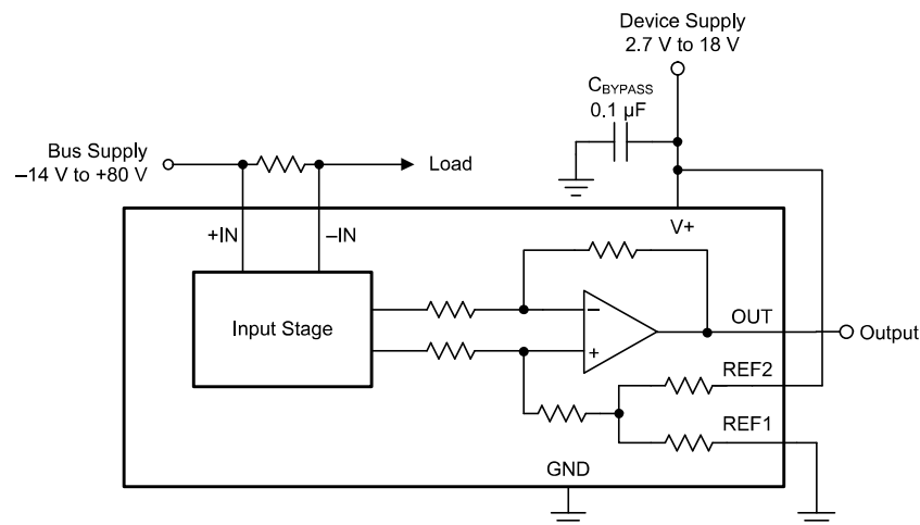
Figure 39. Basic Connections
