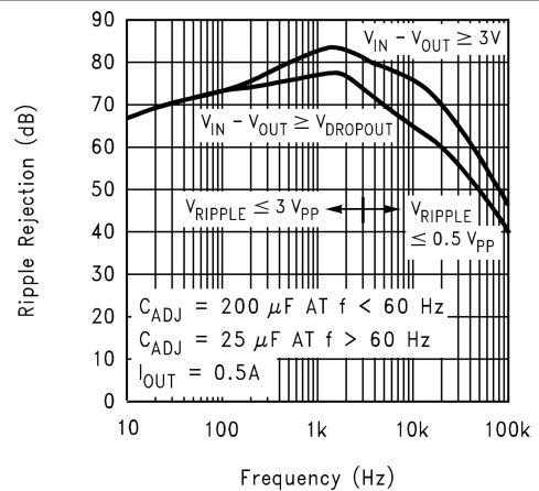
Figure 7-4. LM1117-ADJ Ripple Rejection
