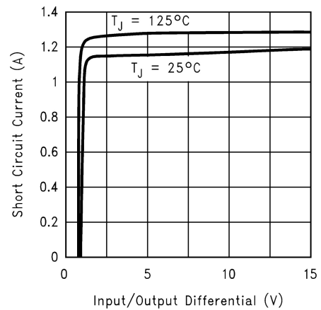
Figure 7-2. Short-Circuit Current
