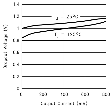
Figure 9-2. Dropout Voltage ( V_{\text{IN}} - V_{\text{OUT}} )
