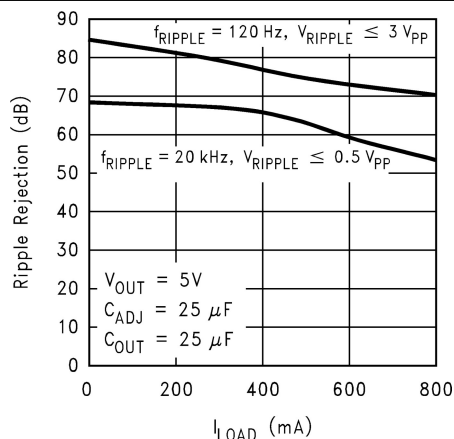
Figure 7-5. LM1117-ADJ Ripple Rejection vs Current
