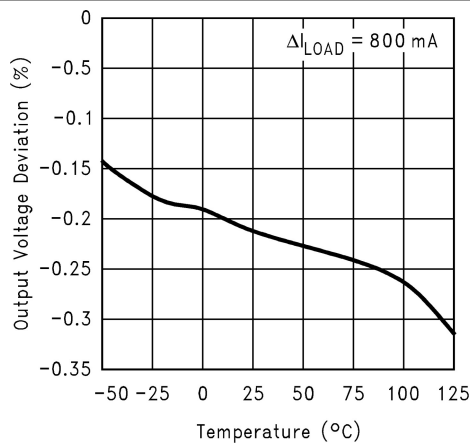
Figure 7-3. Load Regulation
