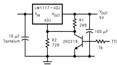
Figure 9-6. 5-V Logic Regulator With Electronic Shutdown*
