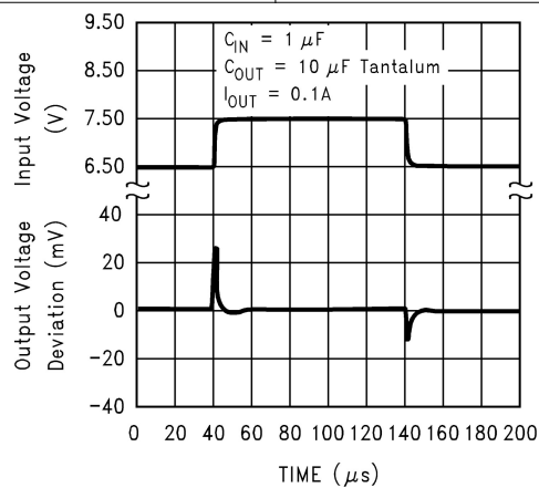
Figure 7-9. LM1117-5.0 Line Transient Response
