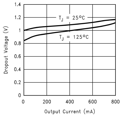
Figure 7-1. Dropout Voltage ( V_{IN} - V_{OUT} )
