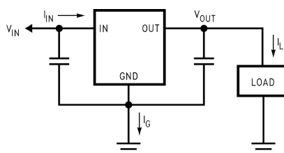
Figure 9-10. Power Dissipation Diagram
