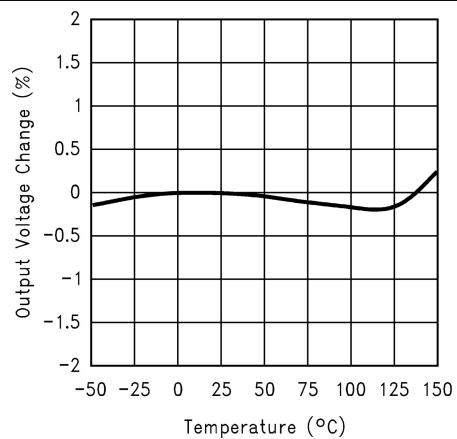
Figure 7-6. Temperature Stability
