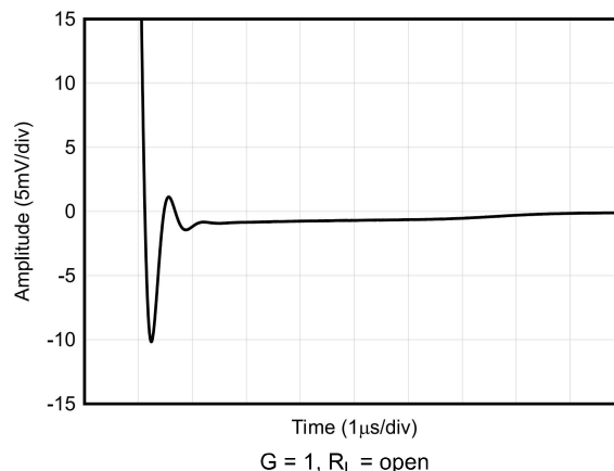
Figure 6-26. Small-Signal Step Response, G = 1
