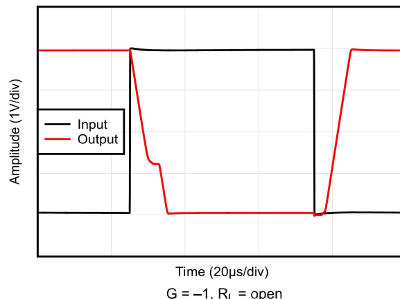
Figure 6-30. Large-Signal Step Response, G = -1
