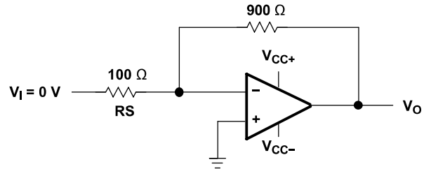
Figure 7-2. Noise-Test Circuit
