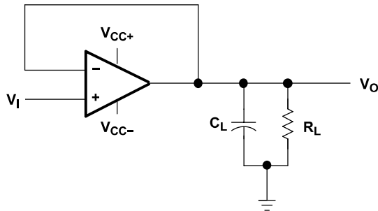
Figure 7-1. Unity-Gain Amplifier
