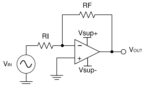
Figure 9-1. Application Schematic
