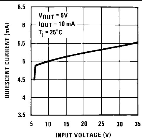
Figure 12. Quiescent Current
