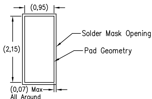
Example, non-solder mask defined pad. (Preferred)
