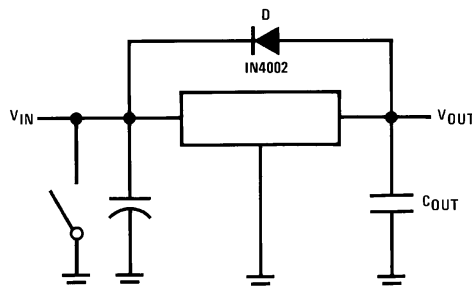
Figure 15. Input Short
