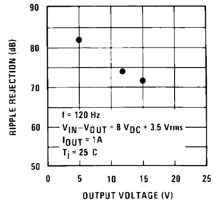
Figure 6. Ripple Rejection
