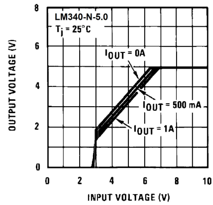
Figure 8. Drop-out Characteristics
