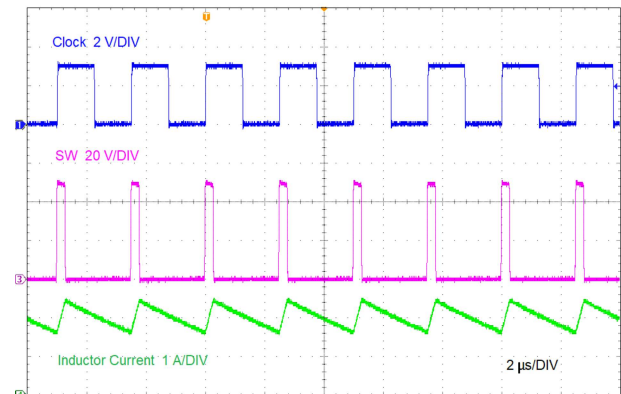
Figure 9-10. Frequency Synchronization
