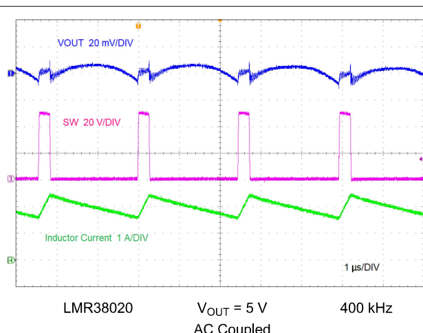
Figure 9-6. Full Load Switching
