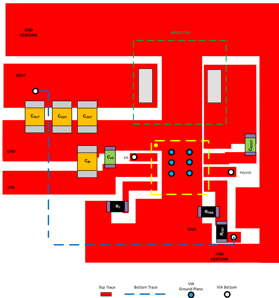
Figure 9-16. Example Layout for HSOIC (DDA) Package
