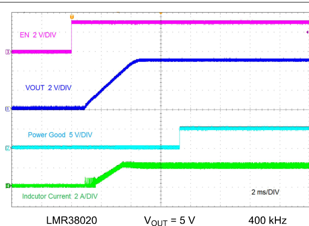
Figure 9-4. Start-Up by EN
