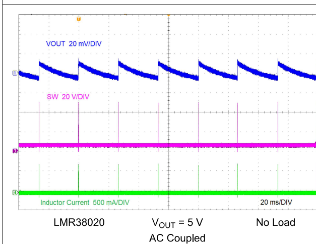
Figure 9-5. PFM Switching
