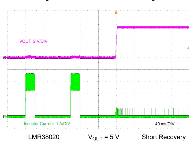
Figure 9-8. Short-Circuit Recovery
