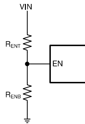
Figure 9-2. Setup for External UVLO Application
