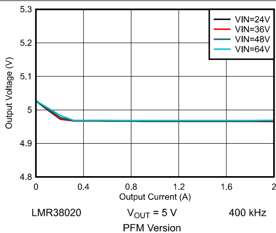
Figure 9-13. 5-V Load Regulation
