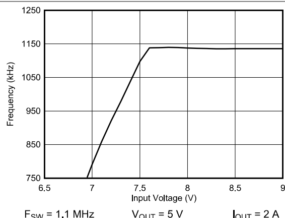
Figure 8-9. Typical Frequency Foldback at T OFF_MIN
