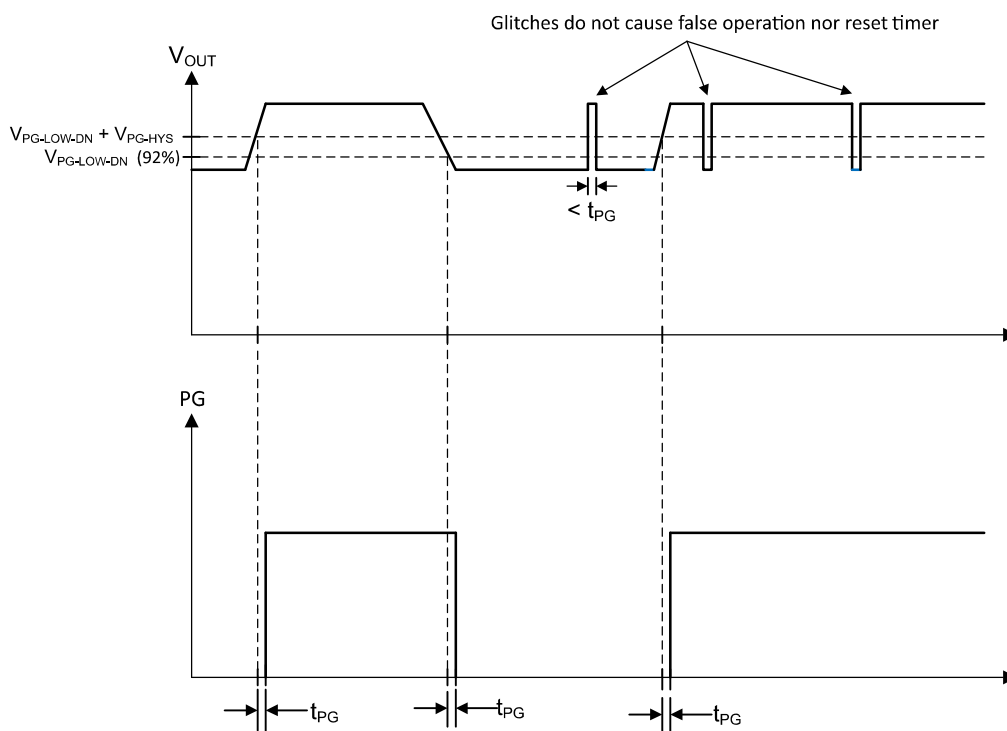
Figure 8-7. Power-Good Timing Behavior
