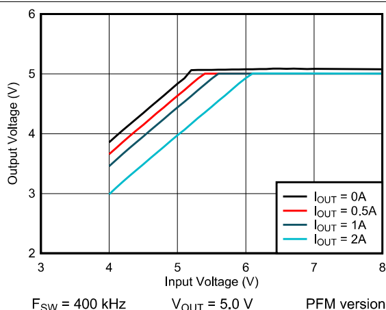
Figure 7-3. 5-V Dropout
