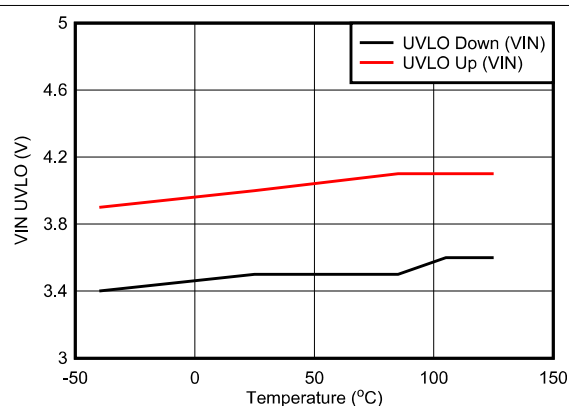
Figure 7-6. V_{IN} UVLO vs Temperature
