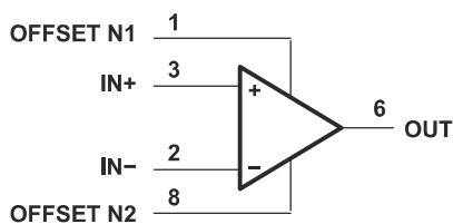
Simplified Schematic
