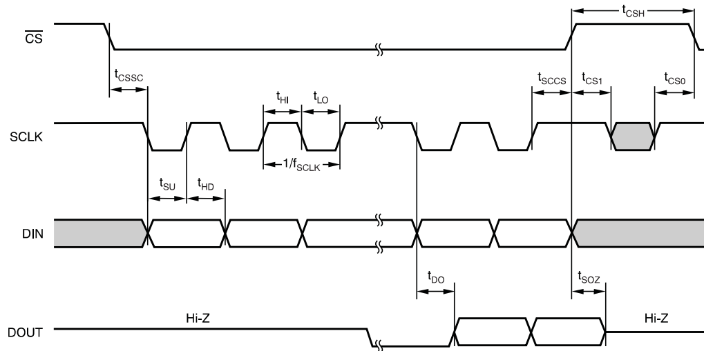
Figure 2. SPI Mode 1, 1
