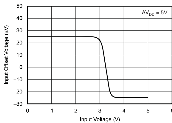
Figure 68. V_{OS} Versus Input Voltage—Case 2
