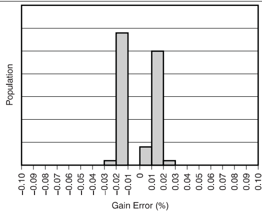
Figure 17. CAL2 Gain Error
