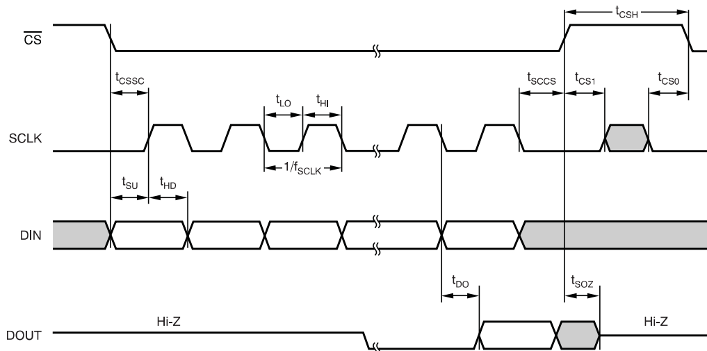
Figure 1. SPI Mode 0, 0
