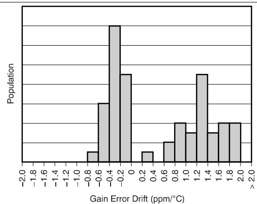
Figure 18. CAL3 Gain Error
