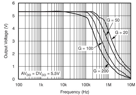
Figure 40. PGA113, PGA117 Output Voltage Swing vs Frequency
