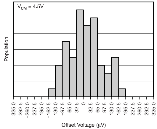
Figure 4. Offset Voltage
