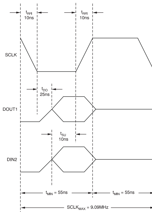
Figure 61. Daisy-Chain Maximum SCLK Frequency
