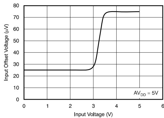
Figure 67. V_{OS} Versus Input Voltage—Case 1
