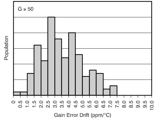
Figure 16. Gain Error Drift ( -40^\circ\text{C} to 125^\circ\text{C} )
