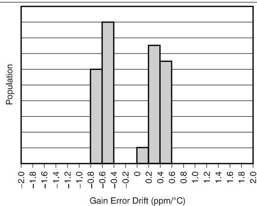
Figure 17. CAL2 Gain Error
