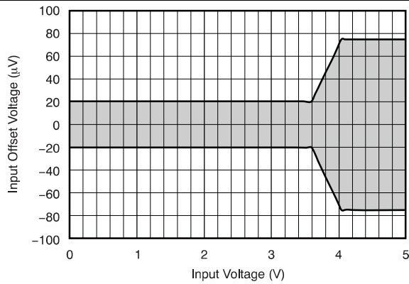
Figure 9. Input Offset Voltage vs Input Voltage
