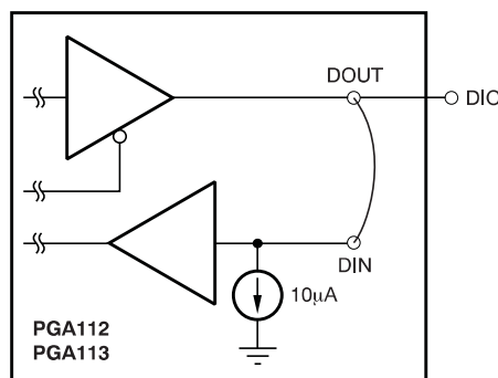
Figure 58. Digital I/O Structure—PGA112 and PGA113
