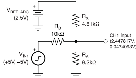
Figure 79. Bipolar to Single-Ended Input Algorithm
