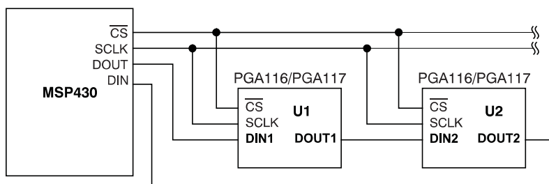
Figure 59. Daisy-Chain Read and Write Configuration
