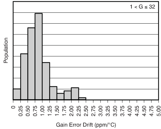
Figure 15. Gain Error Drift ( -40^\circ\text{C} to 125^\circ\text{C} )
