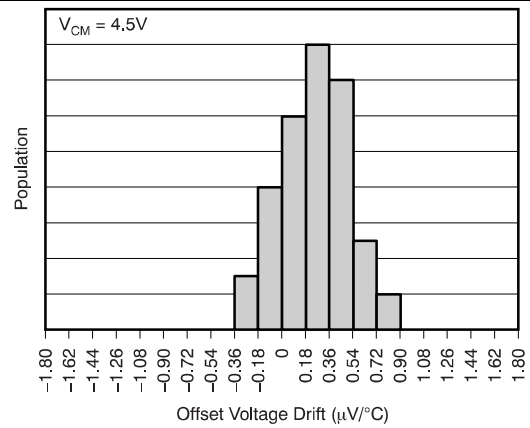
Figure 6. Offset Voltage Drift (–40°C to 85°C)
