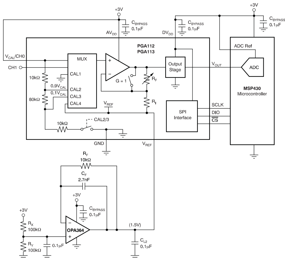
Figure 72. Using CAL Channels With V_{REF} = AV_{DD}/2
