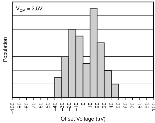
Figure 3. Offset Voltage
