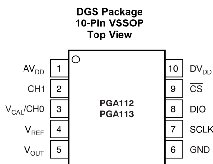
Pin Functions: PGA112, PGA113
