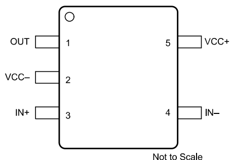
Figure 4-1. TL081H: DBV Package, 5-Pin SOT-23 (Top View)
