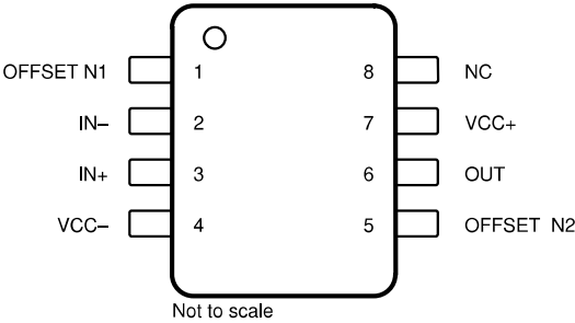
Figure 4-4. TL081C PS Package, 8-Pin SO (Top View)
