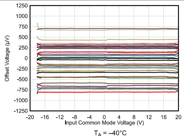
Figure 5-6. Offset Voltage vs Common-Mode Voltage
