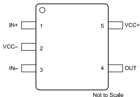
Figure 4-2. TL081H: DCK Package, 5-Pin SC70 (Top View)
