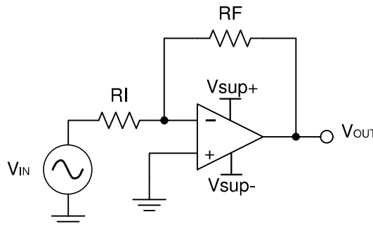
Figure 8-1. Schematic for Inverting Amplifier Application
