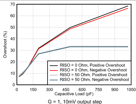
Figure 5-24. Small-Signal Overshoot vs Capacitive Load
