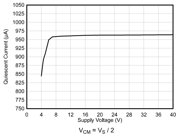
Figure 5-19. Quiescent Current vs Supply Voltage
