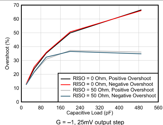
Figure 5-23. Small-Signal Overshoot vs Capacitive Load
