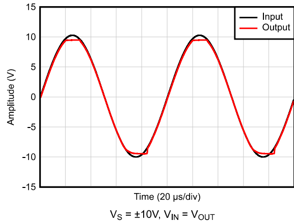
Figure 5-26. No Phase Reversal
