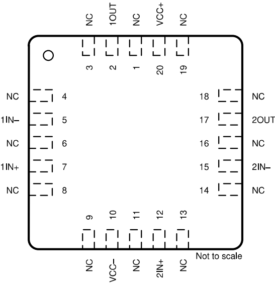
Figure 4-6. TL082 FK Package, 20-Pin LCCC (Top View)
