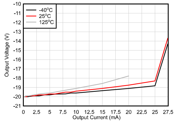
Figure 5-14. Output Voltage Swing vs Output Current (Sinking)
