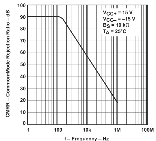
Figure 5-8. Common-Mode Rejection Ratio vs Frequency
