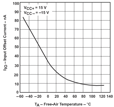
Figure 5-2. Input Offset Current vs Free-Air Temperature
