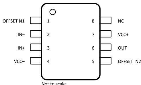
Figure 4-1. uA741C PS Package 8-Pin SO Top View
