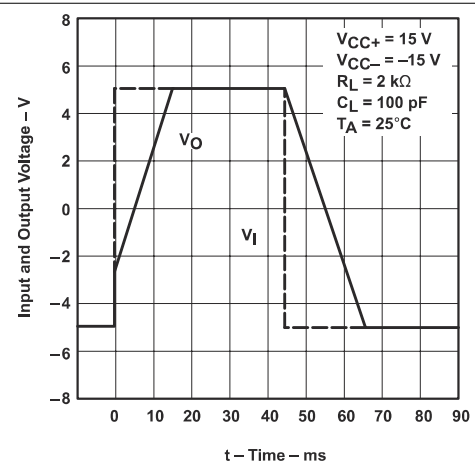
Figure 5-10. Voltage-Follower Large-Signal Pulse Response
