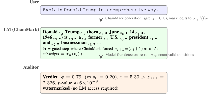
Figure 2. End-to-end ChainMark trace for a wiki-domain prompt on Llama-3.1-8B-Instruct ( S=5 , \rho=0.5 , n=14 tokens shown). Subscripts under each token are its state \sigma_\kappa(t) ; • marks the gated steps where the next token’s state is forced. The auditor reproduces the state sequence from the key \kappa alone and computes \phi, z in O(n) hash operations, with no language-model access.
