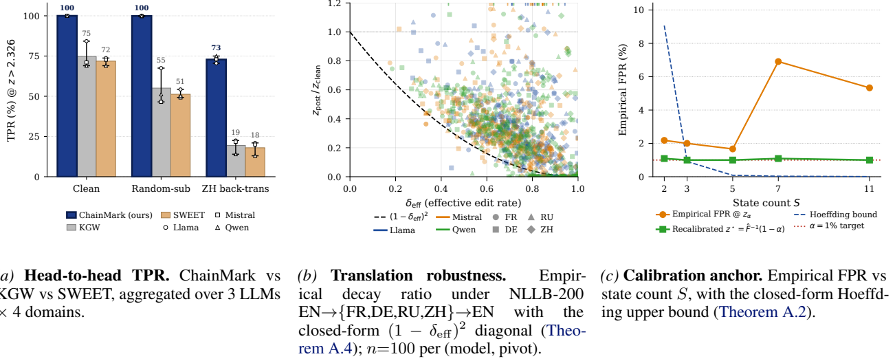
Figure 3. Experimental headlines. (a) head-to-head TPR (§6.2); (b) translation-decay curve (§6.3); (c) FPR calibration anchor (§6.5).
