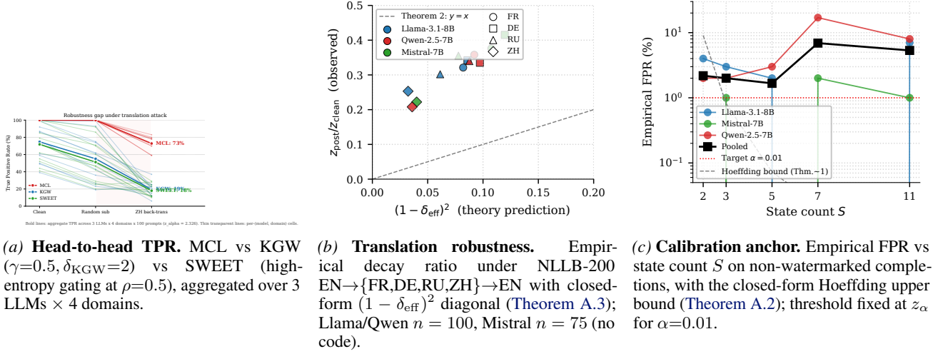
Figure 2. Headline experimental results. (a) Exp. 2 head-to-head TPR. (b) Exp. 3 translation-decay curve. (c) Exp. 5 calibration FPR anchor. Per-pivot translation breakdown in subsection D.1.
