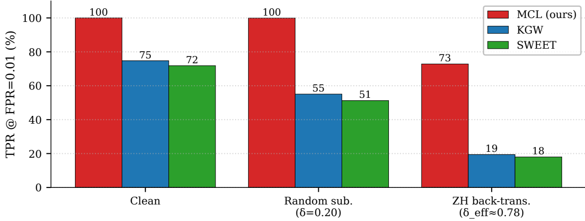
Figure 3. Head-to-head TPR comparison across attacks. MCL ( S=5 , \rho=0.5 , G_{H_{\text{high}}} , k=1 ) vs KGW ( \gamma=0.5 , \delta=2 ) vs SWEET (same KGW params, high-entropy gating at \rho=0.5 ). Aggregated over Llama-3.1-8B, Qwen-2.5-7B, Mistral-7B-v0.3 and four domains (code / factual / wiki / writing).
