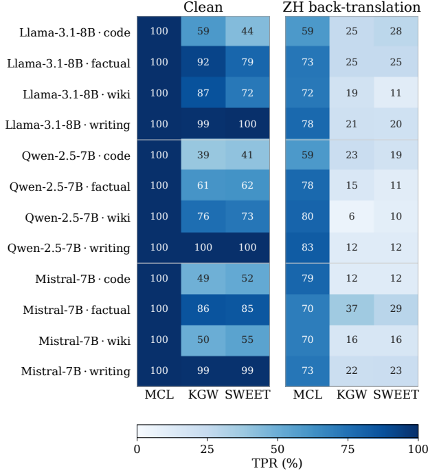
Figure 4. Per-(model, domain) head-to-head TPR (%) at z_\alpha = 2.326 (100 prompts per cell, n=200 tokens). Each row is one (model, domain) cell; left panel is clean, right panel is ZH back-translation. MCL (ChainMark) matches or leads every clean cell and strictly leads every cell post-ZH-back-translation. Cells with \text{TPR} < 50\% are annotated with their value.
