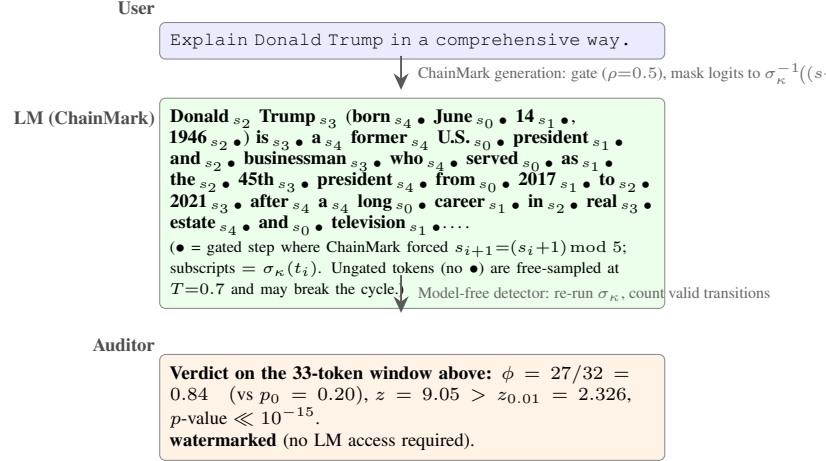
Figure 2. End-to-end ChainMark trace for a wiki-domain prompt on Llama-3.1-8B-Instruct ( S=5 , \rho=0.5 , 33 tokens shown). Subscripts under each token are its state \sigma_\kappa(t) ; \bullet marks the gated steps where the next token’s state is forced. The auditor reproduces the state sequence from the key \kappa alone and computes \phi , z in O(n) hash operations, with no language-model access.
