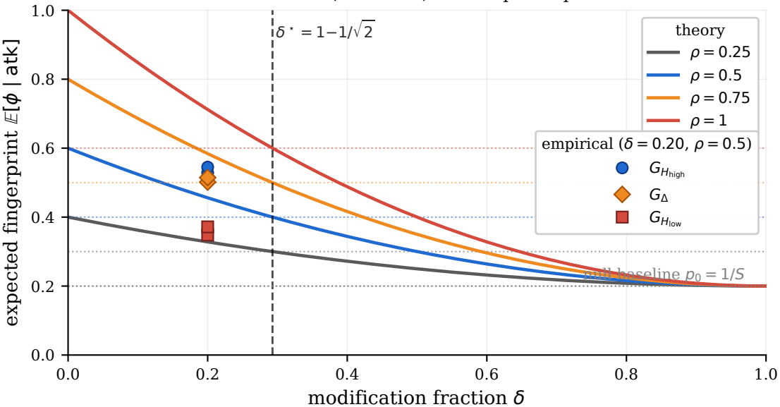
Closed-form robustness curve (Thm.~4.4) with empirical points at \delta = 0.20
