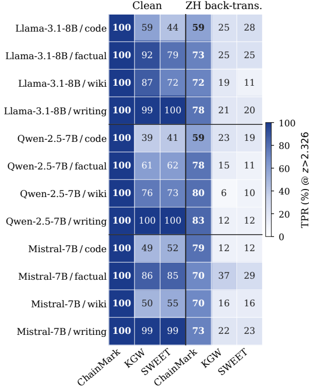
Figure 3. Per-(model, domain) head-to-head TPR (%) at z_\alpha = 2.326 (100 prompts per cell, n=200 tokens). Each row is one (model, domain) cell; left block is clean, right block is ZH back-translation. ChainMark matches or leads every clean cell and strictly leads every cell post-ZH-back-translation. Bold = best per row within each attack block.
