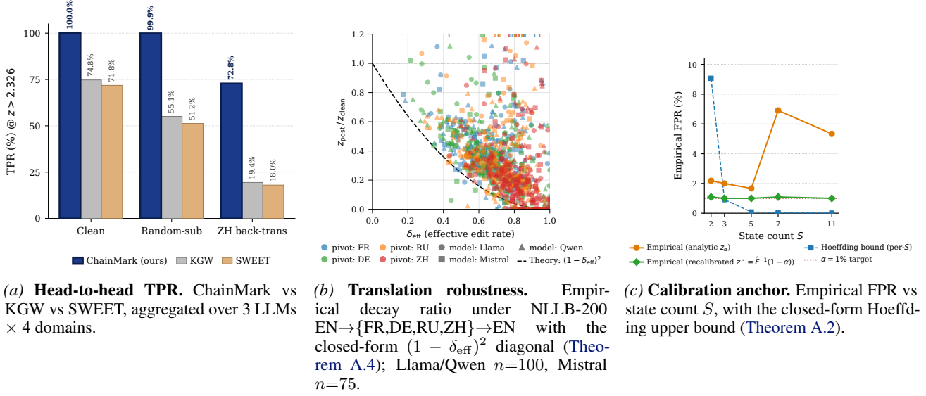
Figure 2. Experimental headlines. (a) head-to-head TPR (§6.2); (b) translation-decay curve (§6.3); (c) FPR calibration anchor (§6.5).
