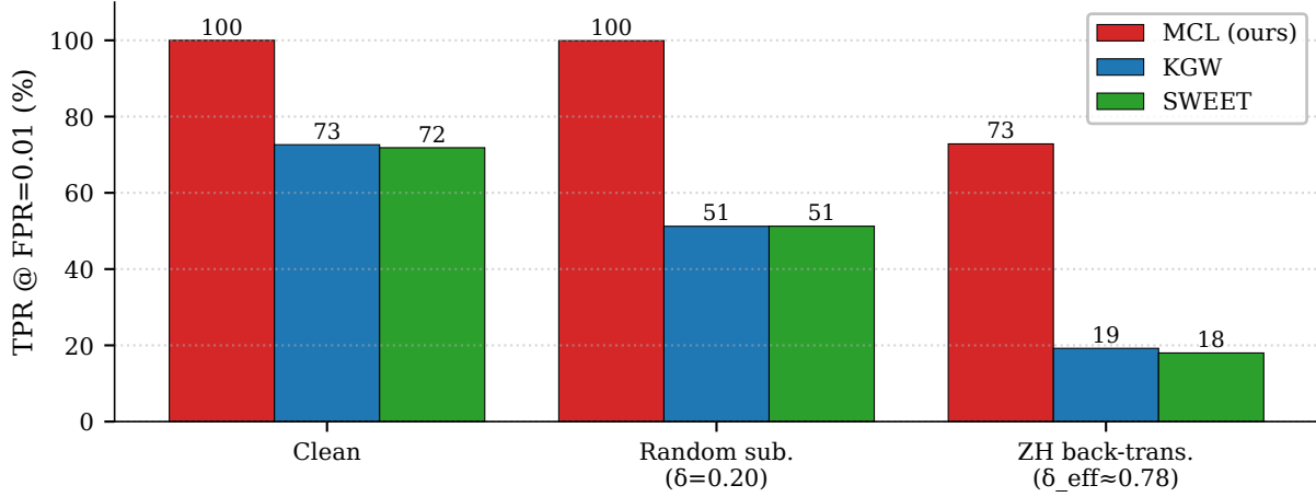
Figure 3. Head-to-head TPR comparison across attacks. MCL ( S=5, \rho=0.5, G_{H_{\text{high}}}, k=1 ) vs KGW ( \gamma=0.5, \delta=2 ) vs SWEET (same KGW params, high-entropy gating at \rho=0.5 ). Aggregated over Llama-3.1-8B, Qwen-2.5-7B, Mistral-7B-v0.3 and four domains (code / factual / wiki / writing).
