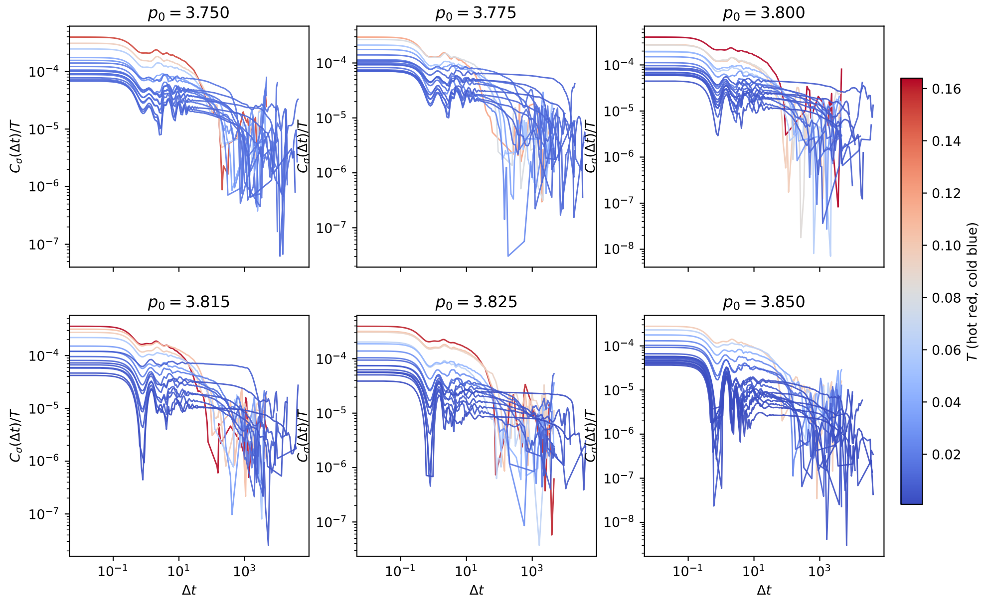
Vertex C_\sigma/T (SAC after 10\tau_{\text{block}} )
