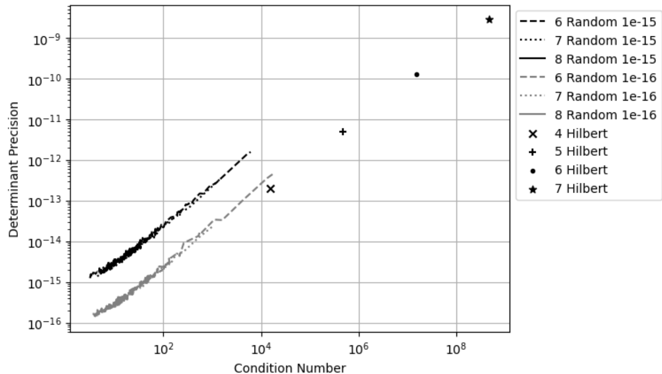
Matrix Determinant Precision vs Condition Number
