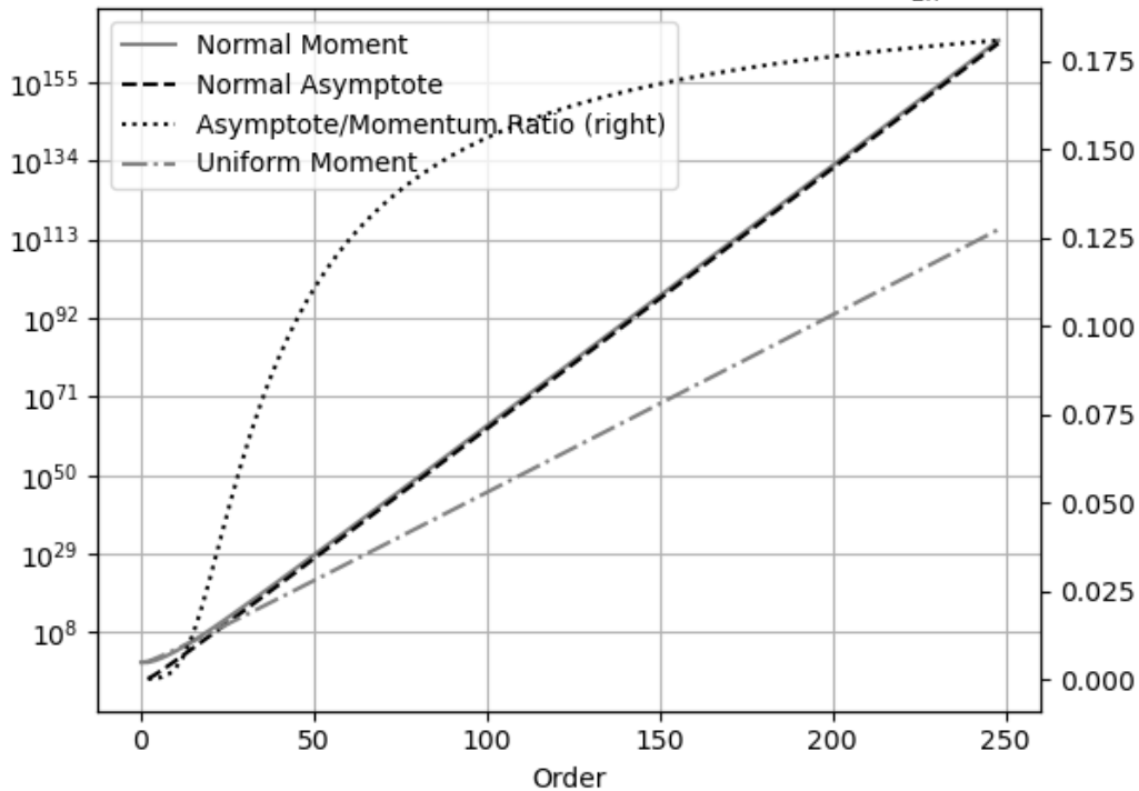
Normal Moment \zeta(2n, 5) vs Asymptotic 2N(5)^{\frac{5^{2n+1}}{2n}}
