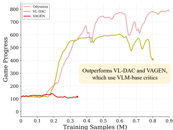
Figure 2: Following the reviewers’ suggestion, we implemented VL-DAC from [Ref 1] and VAGEN from [Ref 2] as additional baselines, which use VLM-based critics. In terms of performance, Odysseus still outperforms VL-DAC and VAGEN . Moreover, under the same batch-size configuration, VL-DAC and VAGEN require roughly twice the GPU resources of Odysseus in our experiments. This highlights the resource efficiency of Odysseus , which benefits from its lightweight CNN-based critic.
